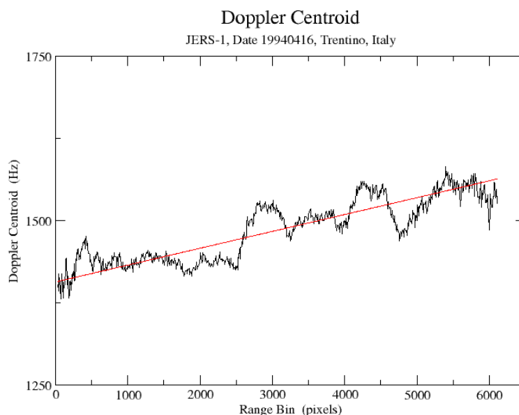
Figure C2. Doppler centroid across swath and linear fit (red line).
